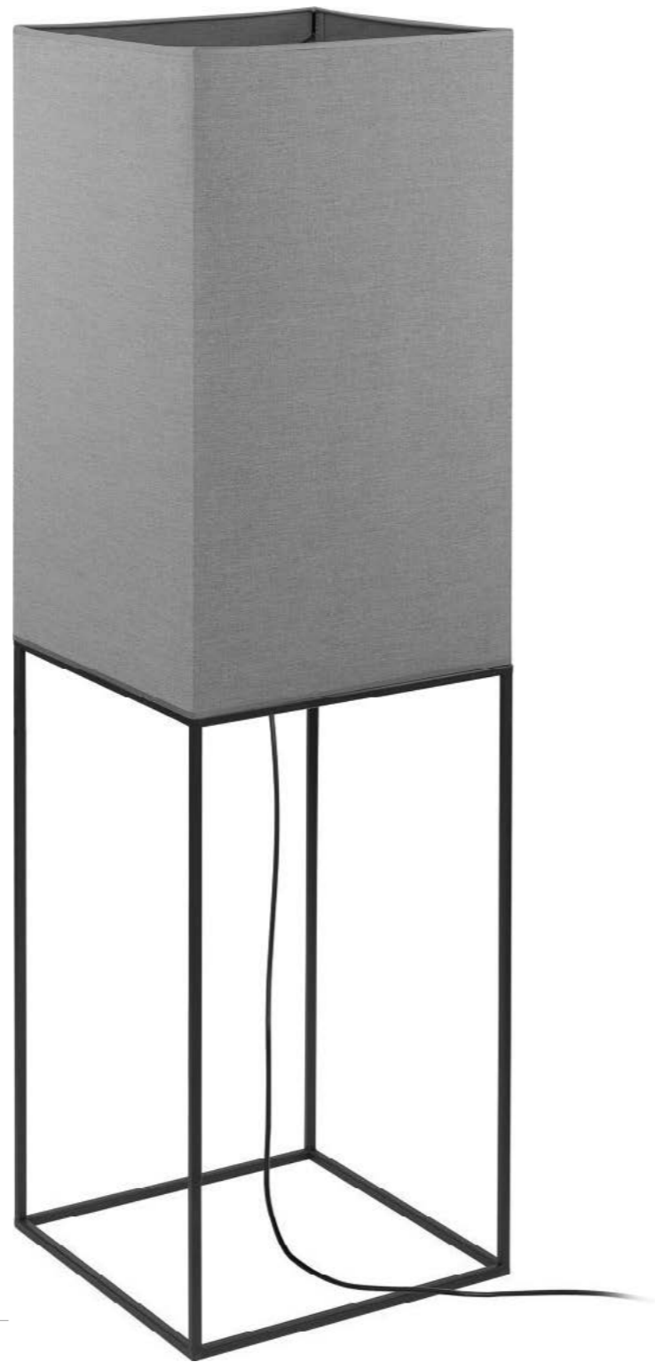
9731 FLAM ↑ 120 cm ↔ 35 cm □ 60 cm 4 x E27, max 60W
